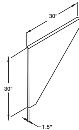
Figure 1 — 6KWL6 Dimensions
