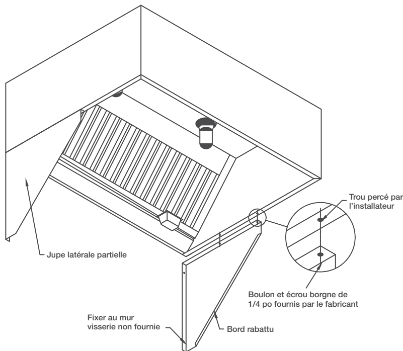
Figure 2 — Pose typique
