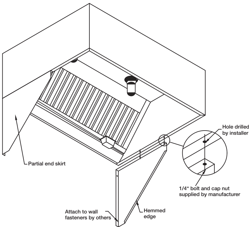
Figure 2 — Typical Installation
