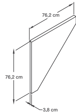
Figure 1 — Dimensions de 6KWL6
